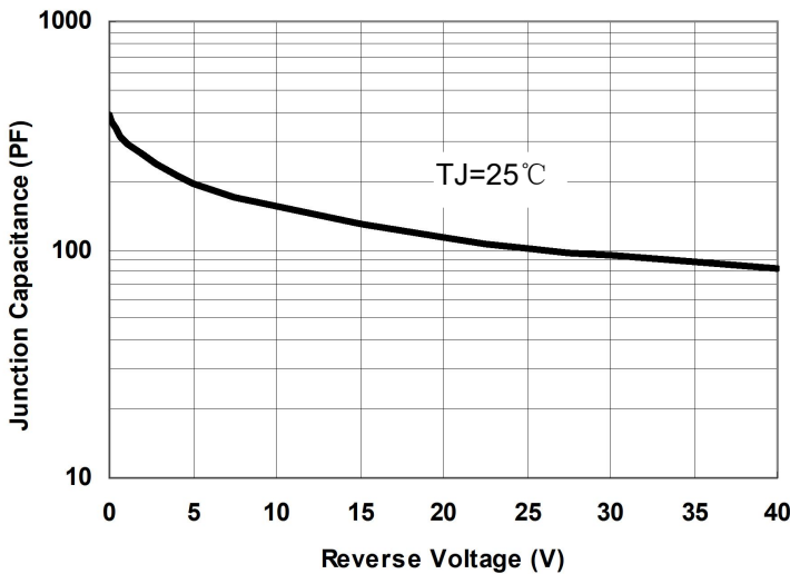
Fig.1-Typical Junction Capacitance
